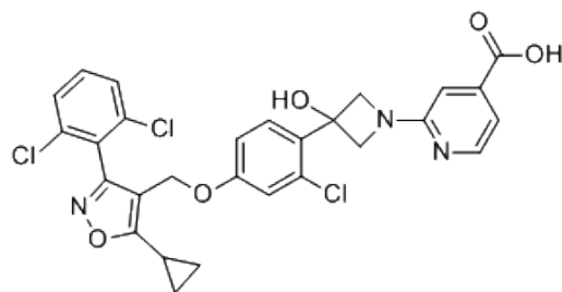
PC-6136801, DMSO-d6
